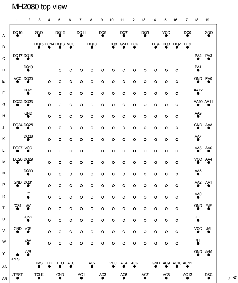
Figure 4: MH 2080 High density Leadless Array (HLA) pinout
